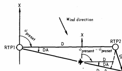
FIG. 54. AIRCRAFT FLIGHT PATH WITH INDEPENDENT DEAD-RECKONING OF COORDINATES IN WIND
